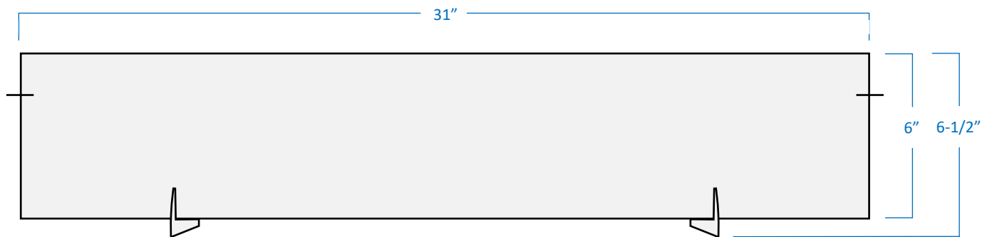
Front View
